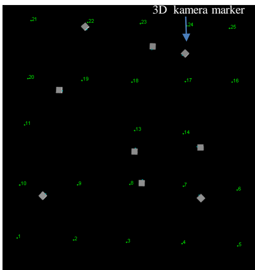
Gambar 3. Kalibrasi In-Field
