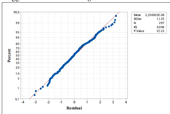
Gambar 2. Plot Residual Berdistribusi Normal
