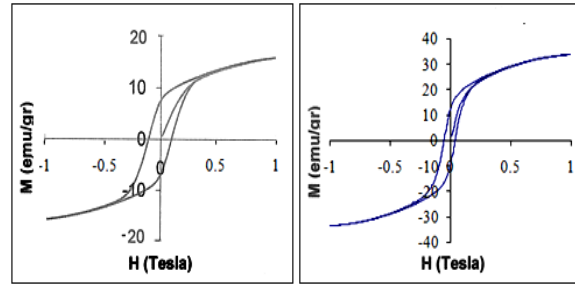
Gambar 4. Kurva Histerisis (a) BAM tanpa Doping dan (b) BAM Doping Ion Zn^{2+}
