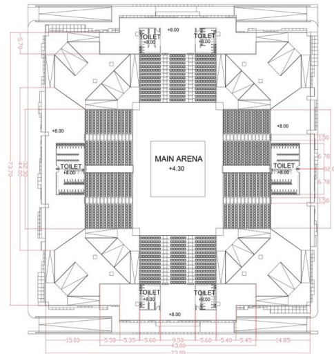
Gambar 13. Denah Lantai 3
