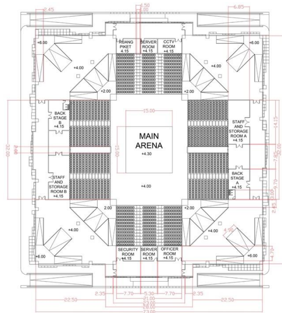
Gambar 12. Denah Lantai 2
