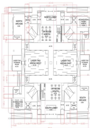
Gambar 11. Denah Lantai 1
