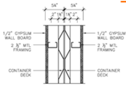
Gambar 4.3 Detail Potongan Dinding Kontainer [7]
