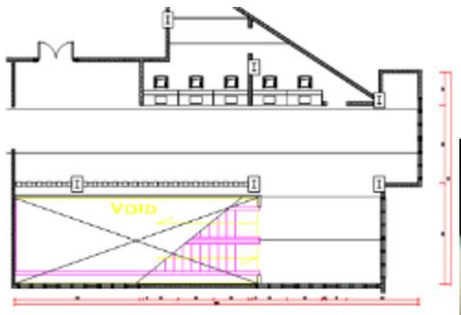
Gambar 4.1. Denah Layout Furnitur – Ruang Ticketing
