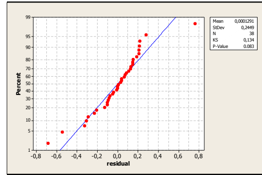
Gambar 4. QQ PLOT
