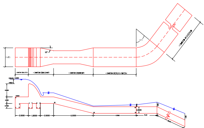
Gambar 4. Desain Spillway
