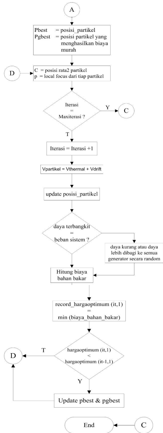
Gambar 4. Flowchart Penerapan RDPSO
