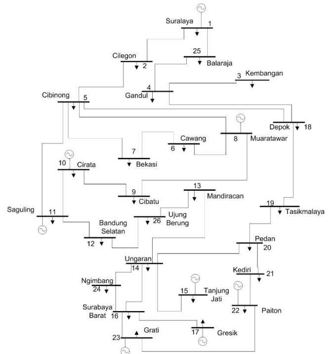
Gambar 3 SLD Jawa Bali 500 kV
