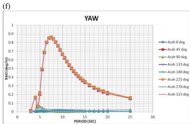
Gambar 4 Grafik RAO kondisi 10% consummables ; (a) surge; (b) sway; (c) heave; (d) roll; (e) pitch; (f) yaw.
