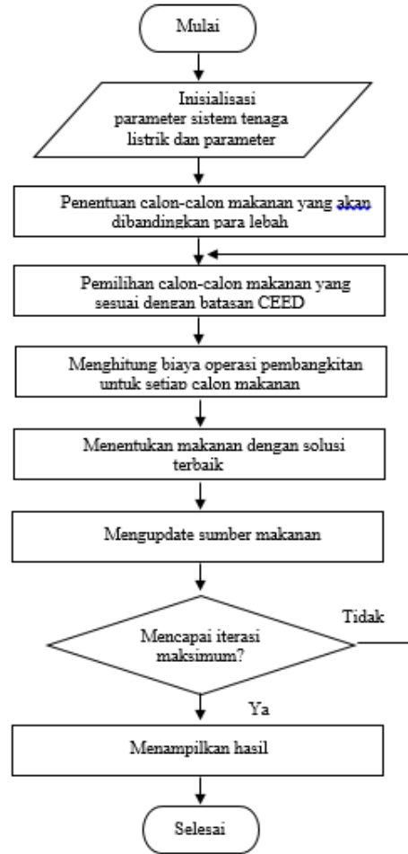
Gambar 4. Diagram Alir Modified Artificial Bee Colony Algorithm
