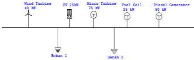
Gambar 1. Tipe microgrid mode operasi islated
