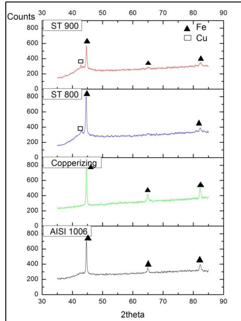
Gambar 5. Hasil XRD Baja AISI 1006, Copperized -AISI 1006, dan Sampel Solution treatment
