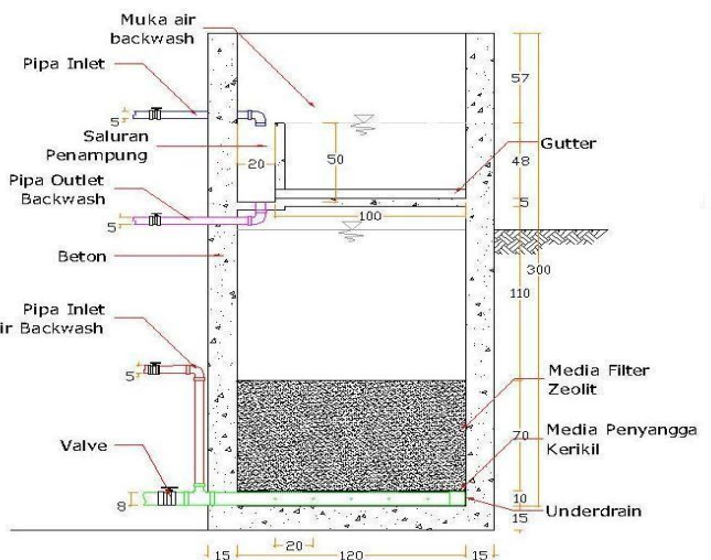
Gambar 7. Potongan Unit Filter Tanpa Skala
