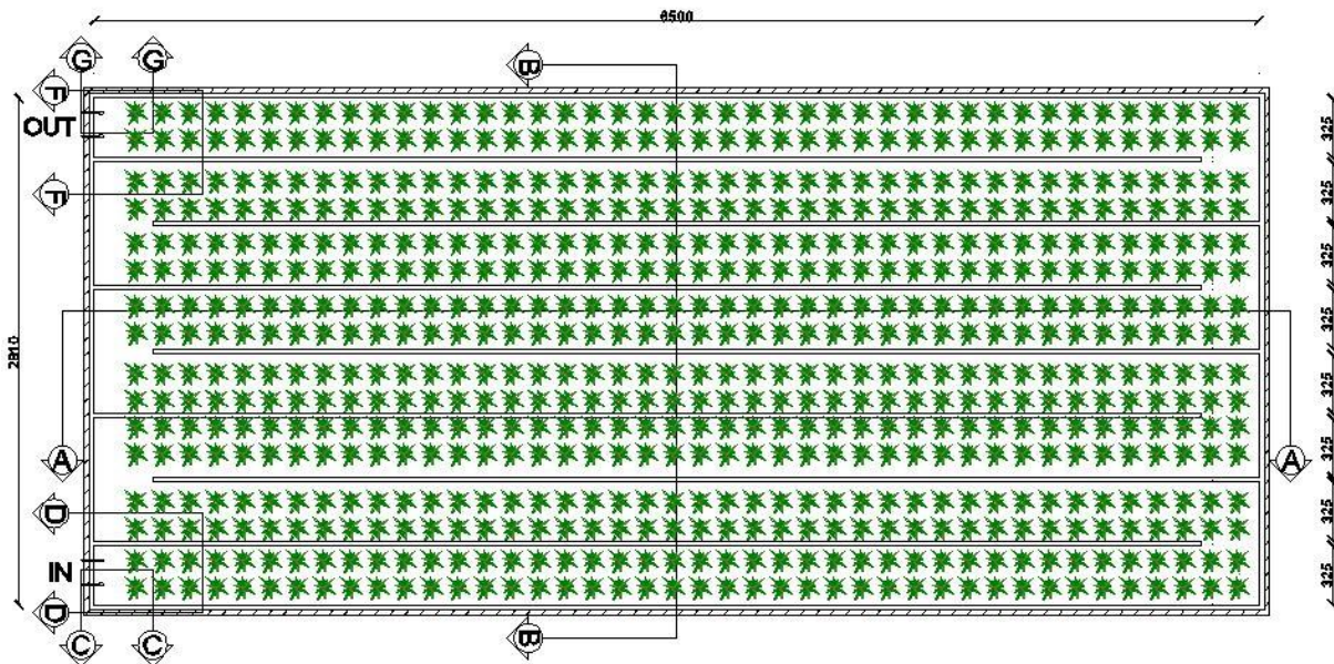
Gambar 7. Denah unit SSFCW
