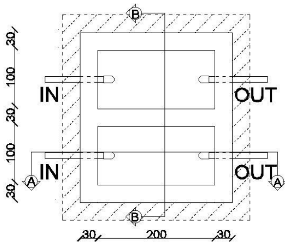
Gambar 9. Denah kolam indikator
