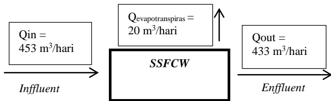
Gambar 4. Water balance evapotranspirasi
