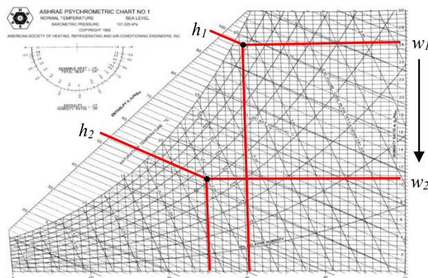
Gambar 5. Grafik Psikrometri proses dehumidifikasi ( h_1 = 97.5 \text{ kJ/kg}_{da} ; h_2 = 54.5 \text{ kJ/kg}_{da} ; w_1 = 26.1 \text{ g}_w/\text{kg}_{da} ; w_2 = 10.5 \text{ g}_w/\text{kg}_{da} )
