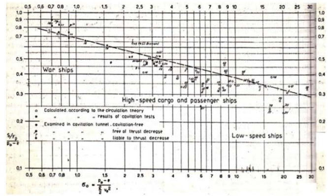
Gambar 3. Diagram bilangan kavitasi
