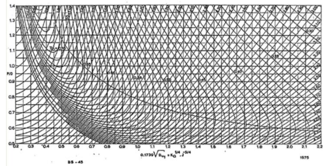
Gambar 2. Contoh diagram propeler B-Troost series
