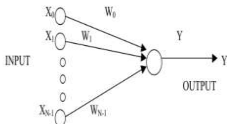
Gambar 5. Model perceptron[10]
