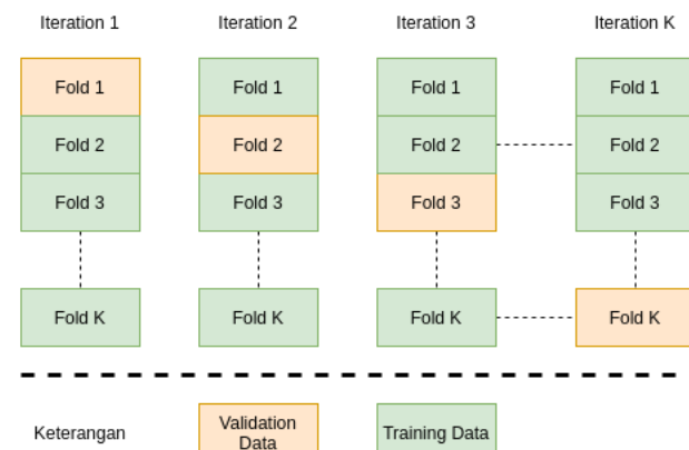
Gambar 9. Visualisasi K Fold Cross Validation .
