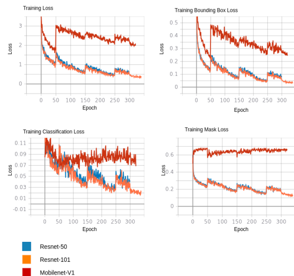
Gambar 11. Grafil perubahan training loss .
