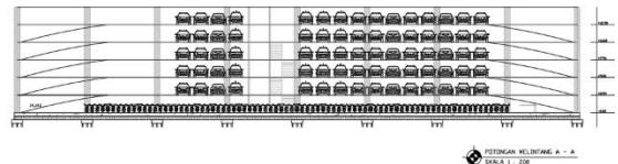
Gambar 6. Potongan Melintang A-A Gedung Park and Ride.
